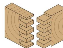
Box joint
